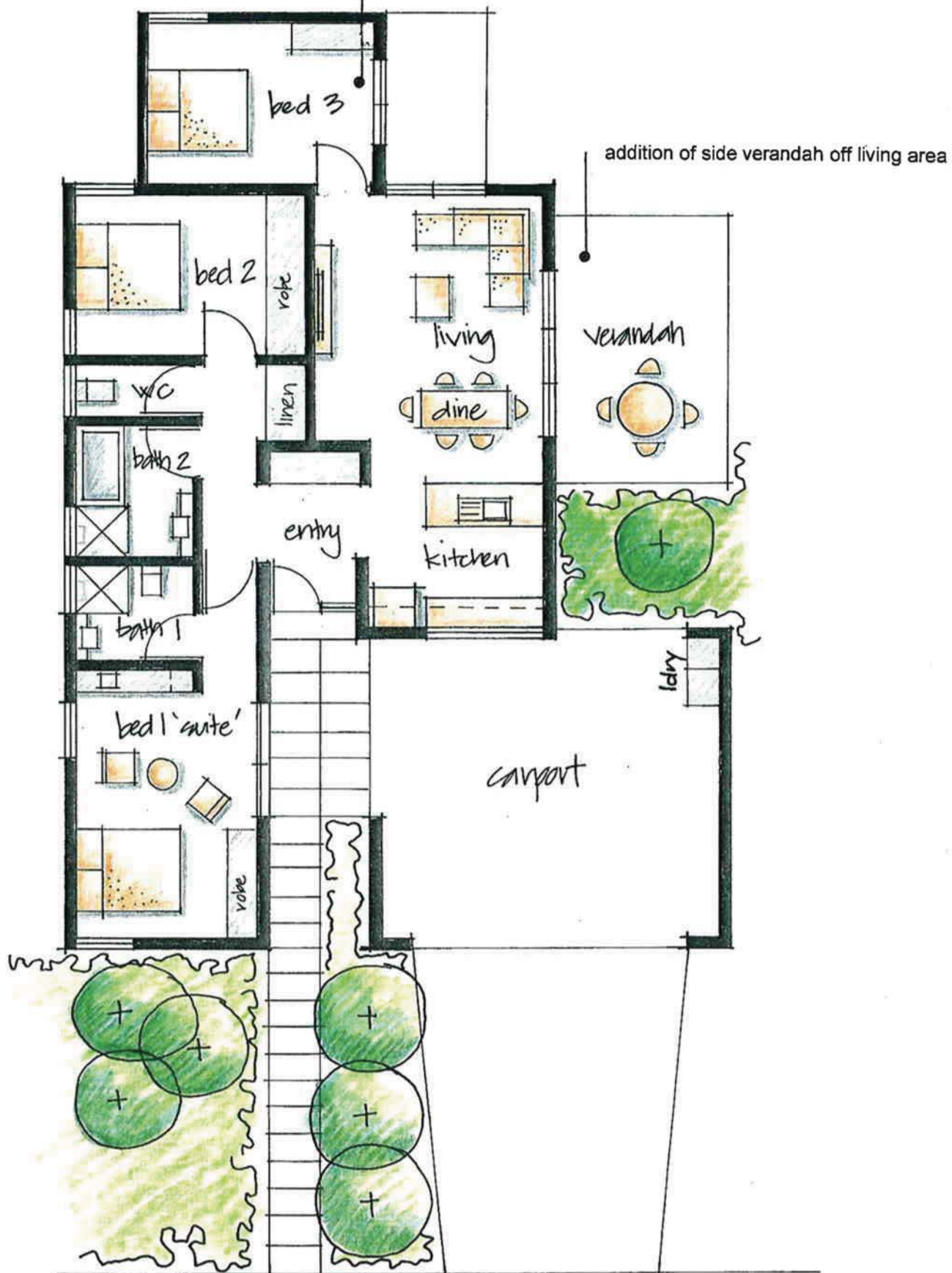
SK06 THREE BEDROOM OPTION (adapted from two bedroom layout)
